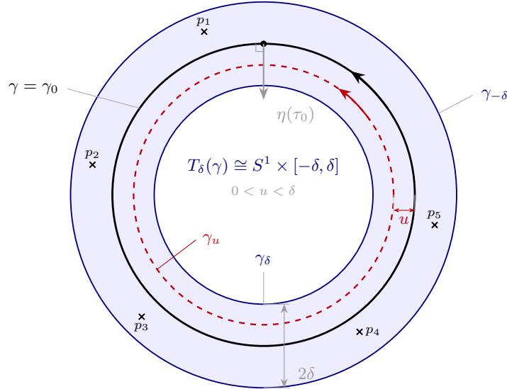
Figure 1: The Fermi strip drawn schematically as an annulus. The central loop \gamma and the parallel curve \gamma_u are closed; positive u points along the chosen normal. The punctures p_1, \dots, p_5 \in S are avoided by the displayed \gamma_u .
